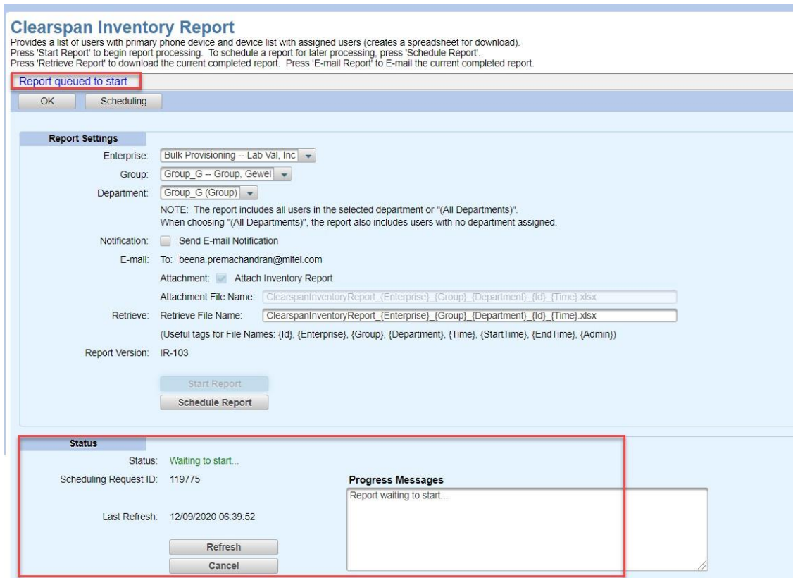
Figure 3: Clearspan Inventory Report Queued – Status Section
